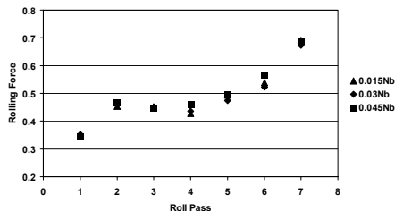
Rolling force per unit width Niobium bearing heats
